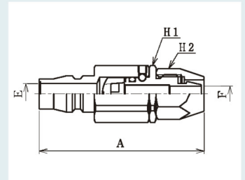
Nut Connection (For Polyurethane Hose) Purge Plug with Rotary Function
