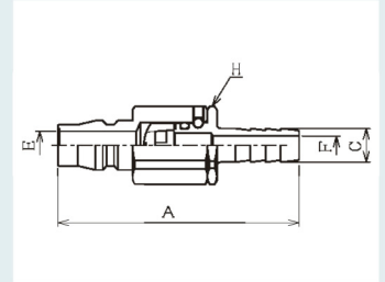
Barb (Hose) connection Purge Plug with Rotary Function
